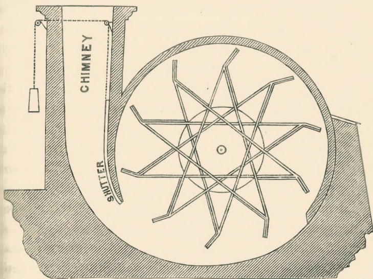
GUIBAL'S FAN.
