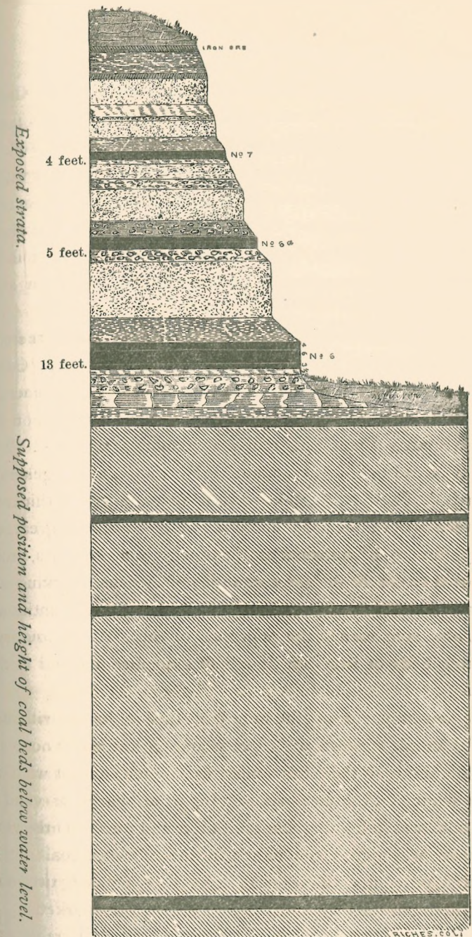
SECTION OF COAL STRATA IN PERRY COUNTY—IN THE VALLEY OF WEST FORK OF SUNDAY CREEK, ON LANDS OF HURD COAL AND IRON COMPANY.
