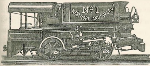
MINE LOCOMOTIVE.
